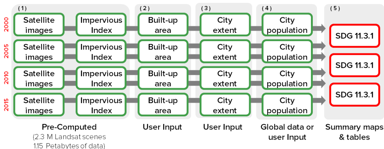
Figure 2: Trends.Earth works-flow to computing SDG 11.3.1. Global 30m impervious surface indices have been pre-computed and are available for the users to explore in the Trends.Earth Urban Mapper where the user defines built-up extent by simply assigning a series of thresholds.
